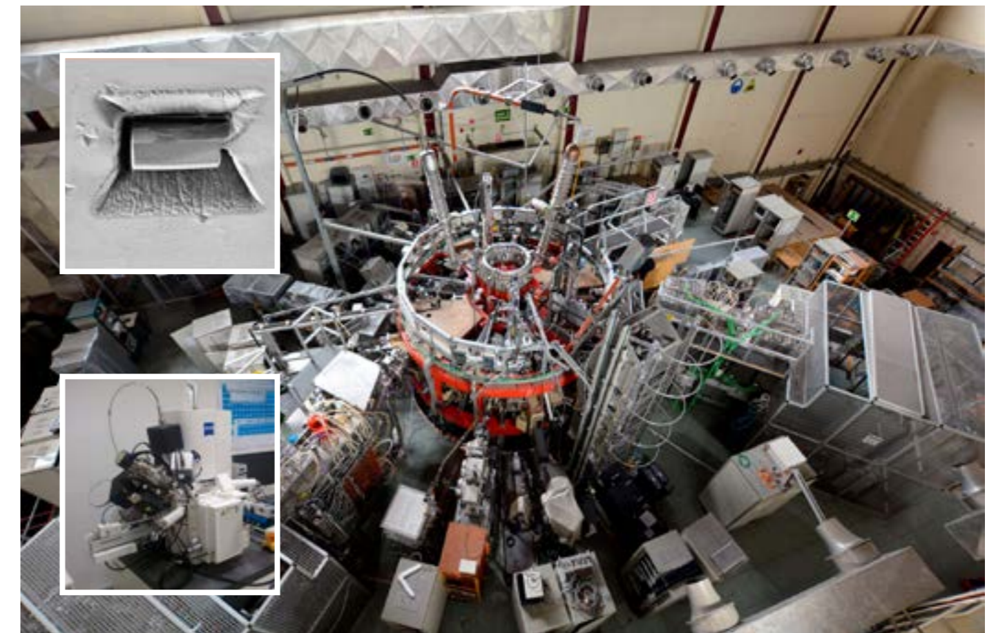
Lower and upper left boxes: manufacture of TEM lamellae at micrometric scale of materials of interest for fusion.
