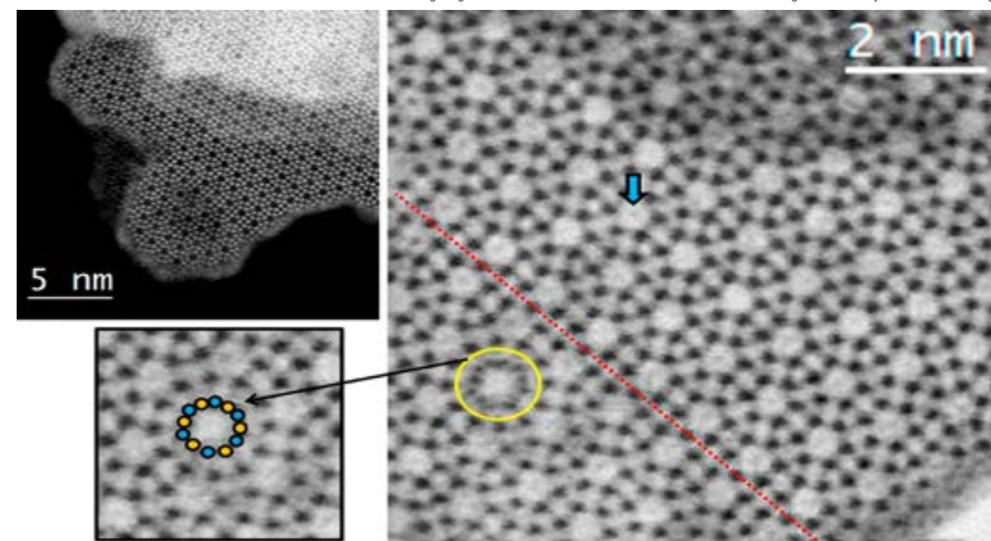
Top left. Atomically resolved HAADF image of a WO 3 nanoplatelet. Bright dots correspond to W atomic columns. The structure is formed by (WO 3 ) n rings stacked along c axis giving rise to tunnels with an internal diameter of 0.48 nm. Right. Atomically resolved ABF image.
