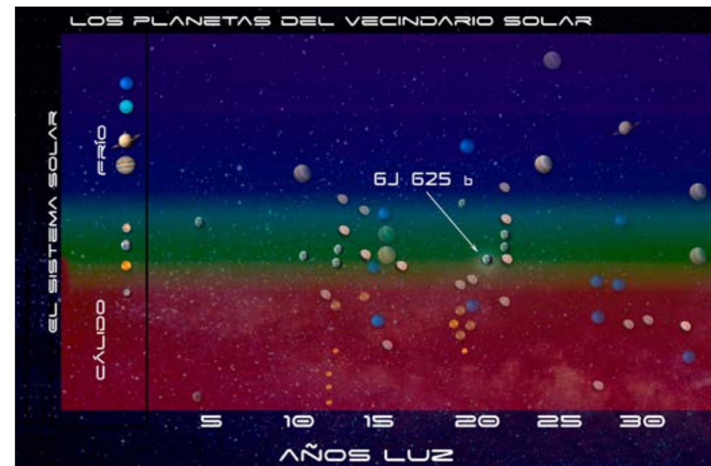
Known exoplanets in the solar neighborhood (up to ~ 35 light years), including the position of GJ 625. The green horizontal region marks the habitability zone. The solar system planets are spotted on the left for comparison
